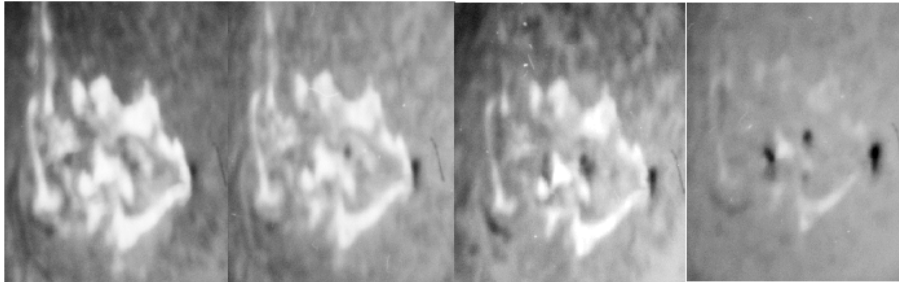
Figure 1: Images of the flare at the H \alpha line center, +0.5Å, -0.5Å, and \pm 1 Å.
