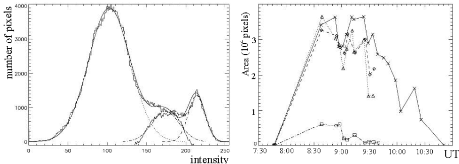
Figure 2: (a) Intensity histogram of a frame at the line center, horizontal axis: intensity level given by the 8-bit camera, vertical axis: number of pixels. (b) Time profiles of the flare at the four wavelengths studied.
