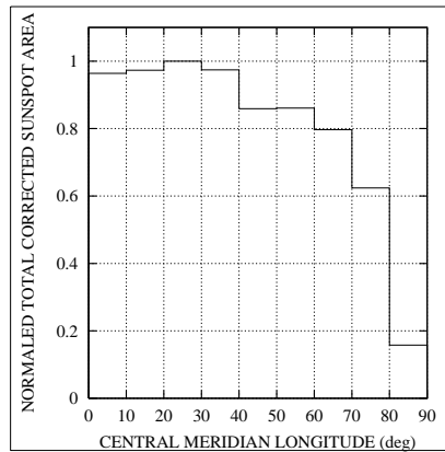
Fig. 3. The normalized total corrected DPD sunspot areas plotted in 10^\circ central meridian longitude belts for 1988, 1989, 1993, 1994, 1995, and 1996.
