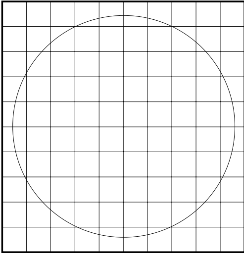
Fig. 4. A circular sunspot on the CCD matrix.
