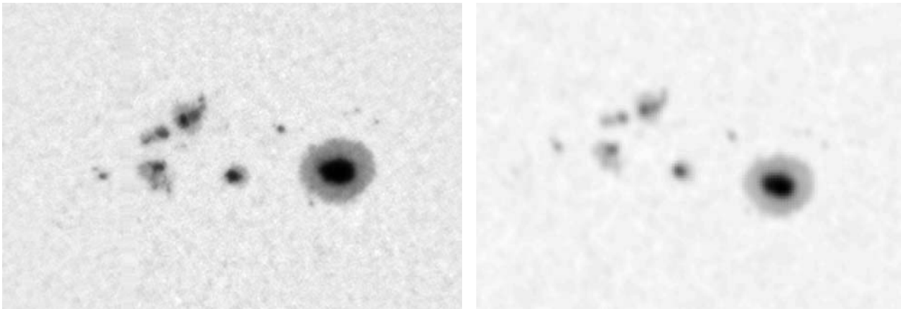
(a) DPD photoheliogram observed in Debrecen at 14:31 UT.
