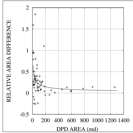
Fig. 5. Relative sunspot area difference versus DPD sunspot area. The continuous line is the function described by equation 2.
